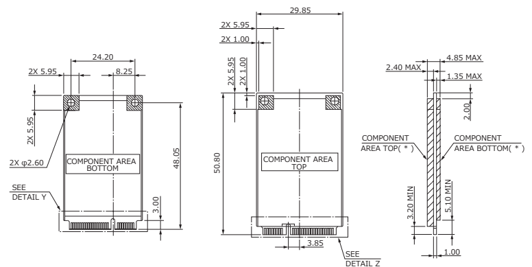
Package view
